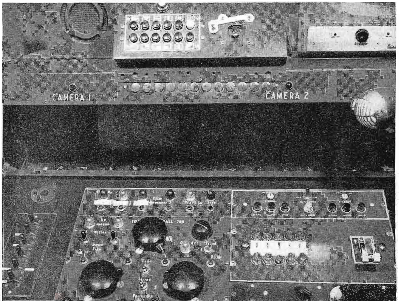
FIG. 15. Closeup of WISH-TV subcontrol console showing Technical Director's position. At top is control panel for video effects equipment. Keys at left for plant intercom. Center panels for remote control of monochrome projector No. 3, slides, and opaques. Right hand panels from top to bottom: projector controls for color projectors, TS-5 switcher, and switching panel (black and white knobs) for connecting video into effects equipment.
