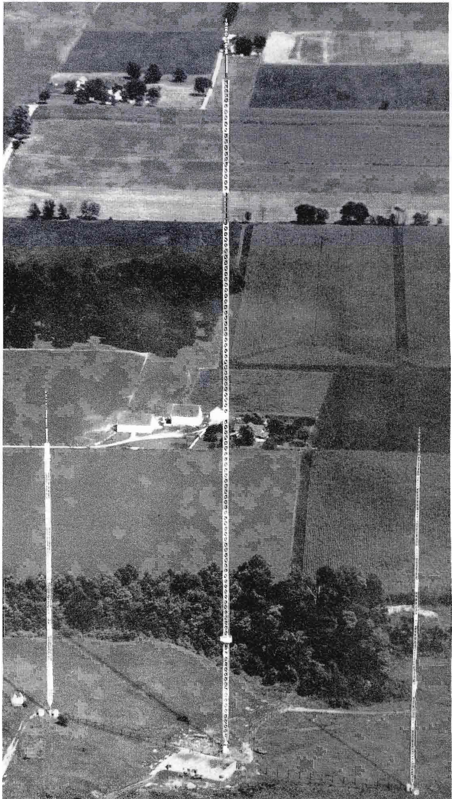
FIG. 7. Aerial view of transmitter site looking east. 1,000 foot TV tower in center. Other towers are 570 feet. Tower at left mounts the emergency TF-12AH antenna for WISH-TV. Regular antenna on 1,000 foot tower is TF-12BH. Although clearly discernible in picture, the center tower is electrically non-existent in the night-time directional array.
