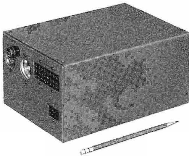
FIG. 13. Compact auxiliary control box houses all relays, drum and mirror motor capacitors.
