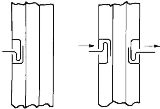
FIG. 5. For the elimination of undesired excitation of the pole the system can be changed from unsymmetrical (left) to symmetrical (right) by using radiators in pairs opposite to each other and in opposite phase. To maintain coupling as purely inductive as possible, the coupling loops are capacitively shielded.
