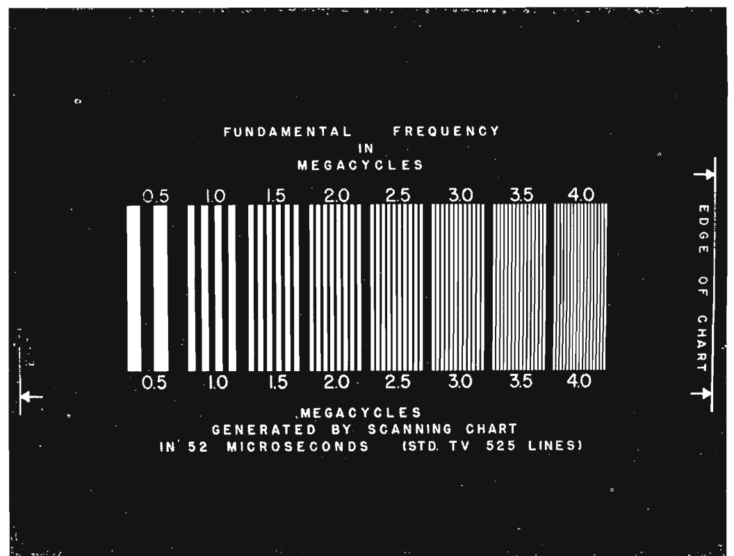
FIG. 15. Special RCA Aperture Test Chart.
