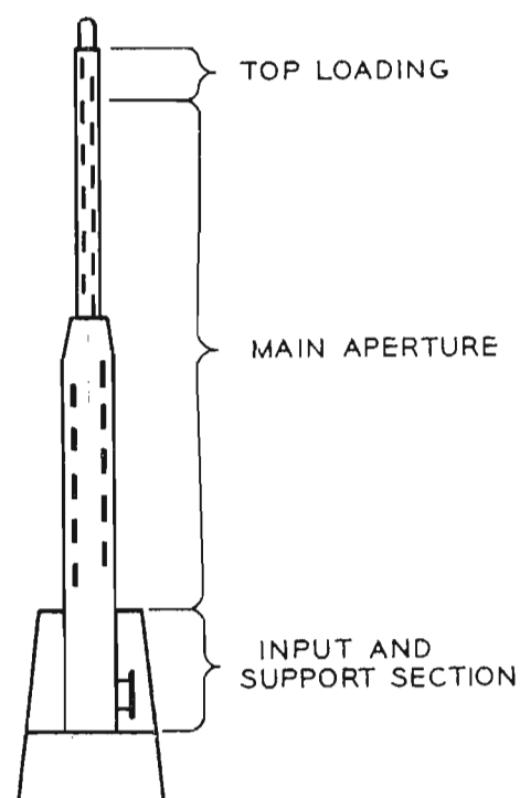
FIG. 1. Outline of the Traveling Wave Antenna.
