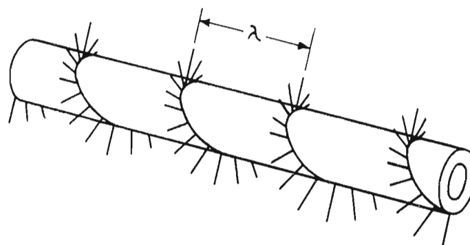
FIG. 4. Antenna having radiators located around the coaxial line on a spiral which has the pitch equal to the wavelength in the line. It has rotating radiator current phase around the periphery and provides an omnidirectional pattern with the main beam perpendicular to the axis of the array.
