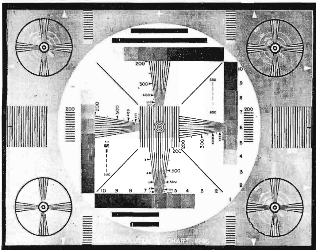
FIG. 10. RETMA Resolution Chart.
