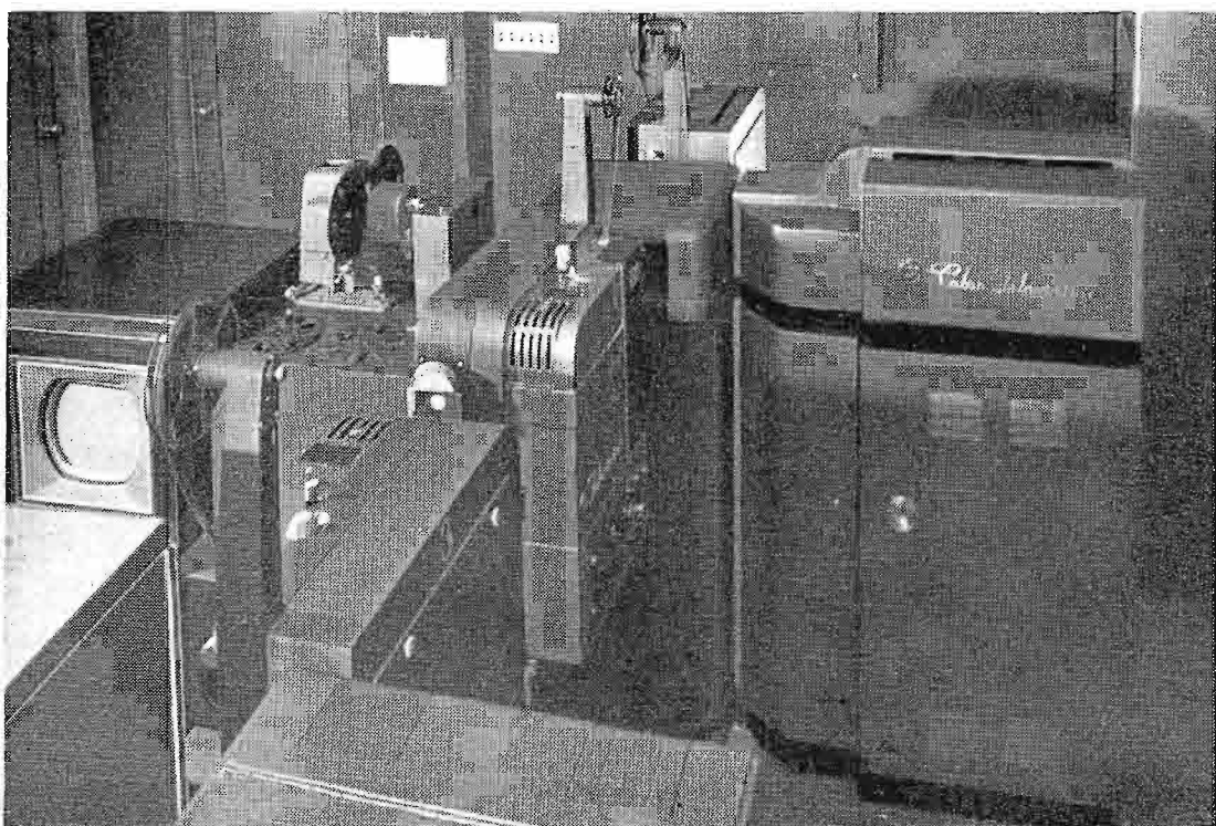
FIG. 17A. View of WISH-TV projection equipment. In foreground, TK-20D iconoscope camera. In background, TP-3 slide projector, TP-15 multiplexer, and TK-26 3-V color camera.
