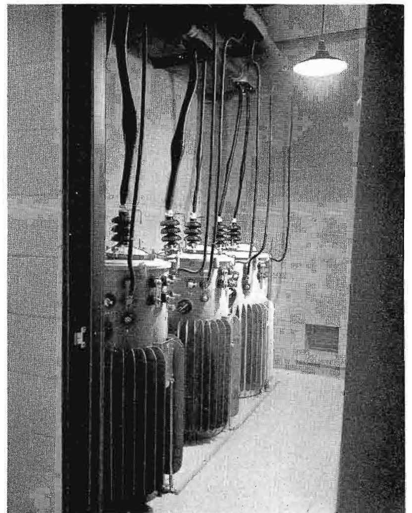
FIG. 8. Although the high-voltage plate transformers are weatherproof and can be mounted outside the building—KSTP chose to install them in a transformer vault. These are the only external transformers which require additional floor space. Note the individual temperature indicators on the transformers.
