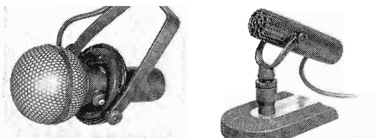
BK-5A Microphone with Wind Screen and new, improved Boom Mount. BK-5A mounted on Type 91-C Desk Stand.
