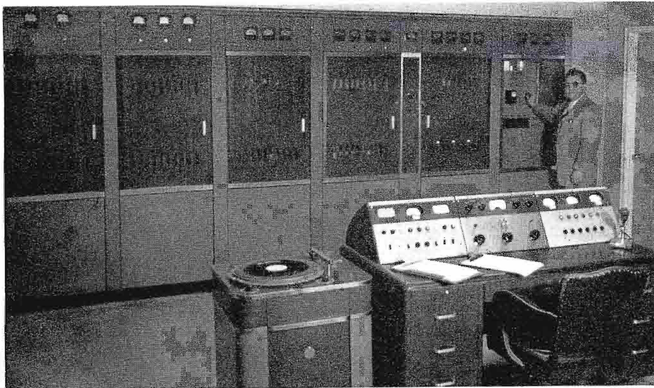
FIG. 5. View of BTA-5H AM transmitter and console. Two cabinets at left are phasing equipment. Right-hand console turret contains control for switching each of the three AM transmission lines to a spare line. Engineer in picture is B. J. Weimer, Transmitter Supervisor.
