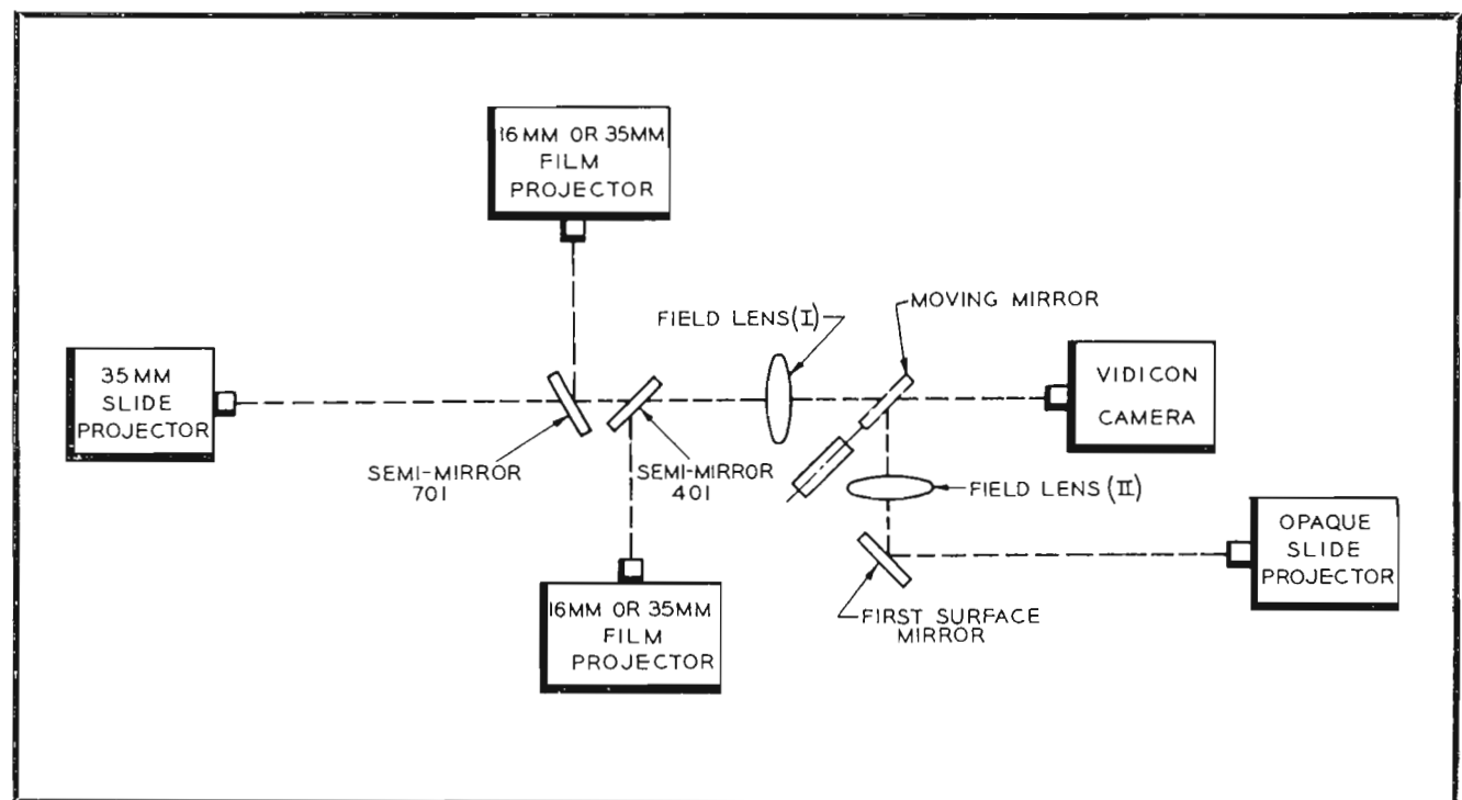
FIG. 2. Optical schematic of TP-11A Multiplexer.
