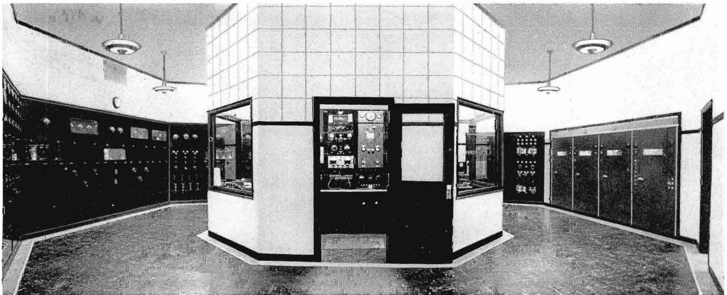
FIG. 1. Interior of transmitter building at KSTP looking toward the rear of the octagonally shaped room. At the far right, the four cubicles of the BTA-50G 50 KW AM Transmitter can be seen. Just to the left of the BTA-50G is a composite 1-kw stand-by transmitter housed in two cabinets. The control room at the center of the main transmitter room contains the transmitter test and measuring equipment as well as facilities for programming of records and station breaks. At the left of the control room, a portion of the old composite 50-kw AM transmitter can be seen. This composite 50-kw unit takes up approximately one-half of the wall space of the transmitter room. In contrast to this, the new BTA-50G occupies less than 15 feet of wall space—an area formerly occupied by a 10-kw FM transmitter.
