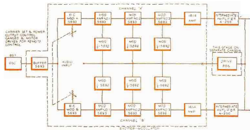
SIMPLIFIED BLOCK DIAGRAM—BTA-50G TRANSMITTER
