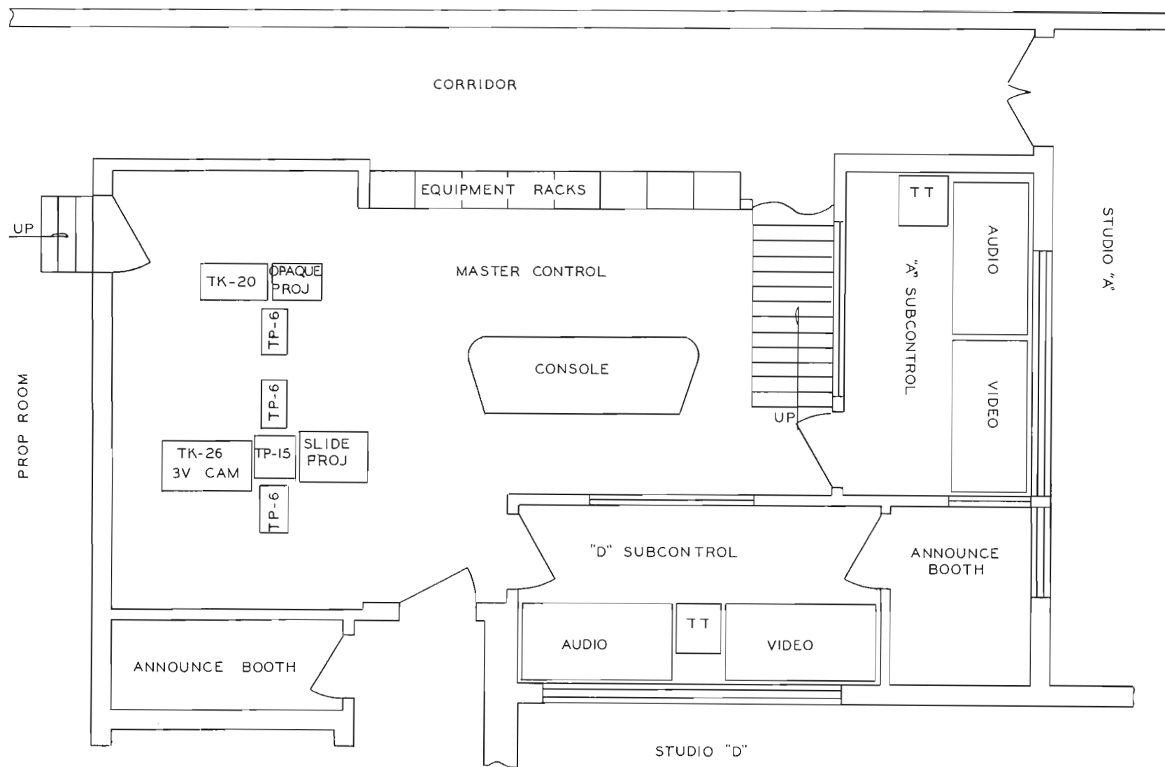
FIG. 18. Floor plan TV control area.
