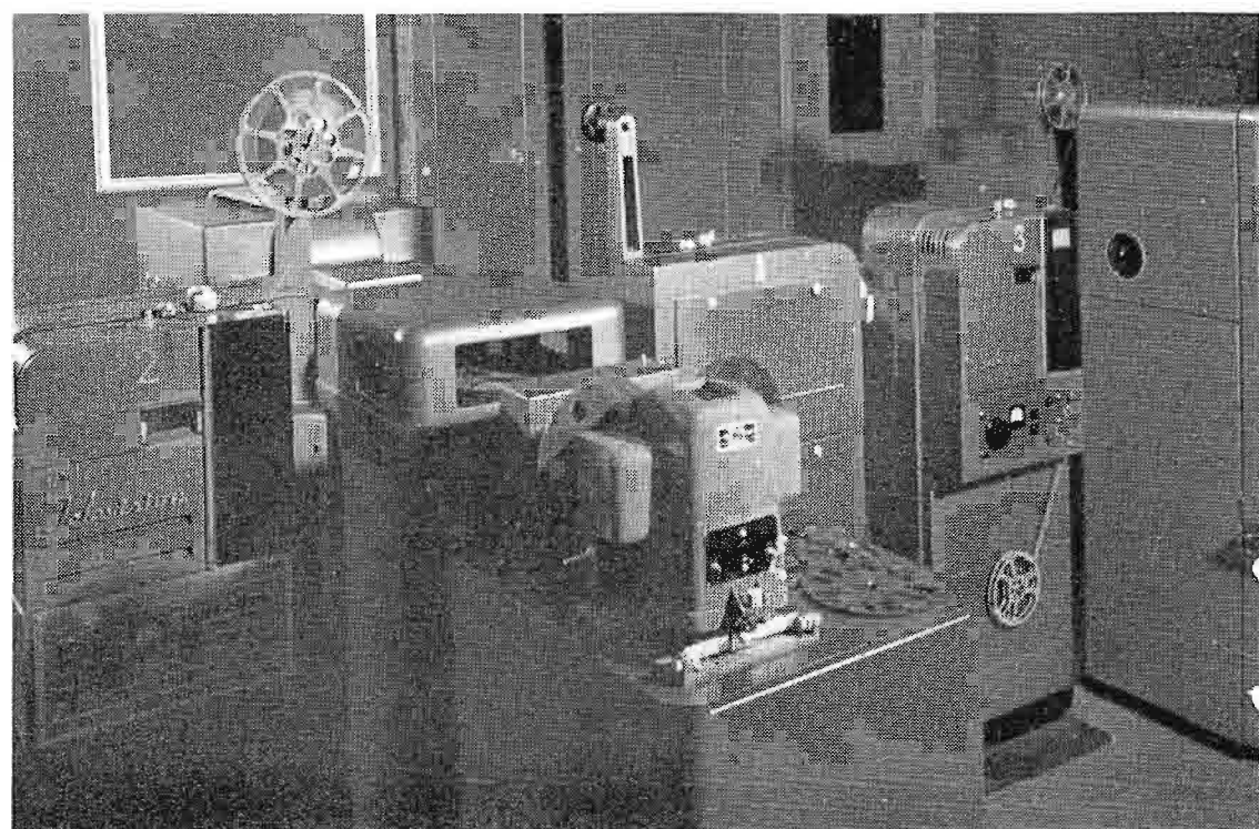
FIG. 17B. View of WISH-TV projection equipment. At left are color film facilities. At right are monochrome facilities. At extreme right is Projectall for slides and opaques.
