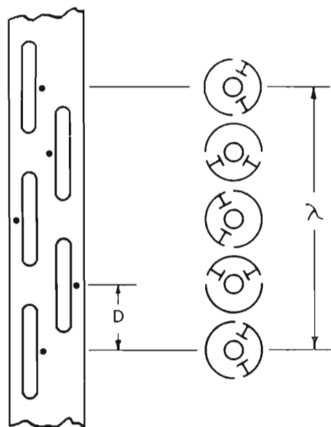
FIG. 2. Simplified drawing shows a portion of the main aperture and its cross-sections at the center of each slot pair. The successive slot pairs are spaced electrically a quarter wavelength apart ( D ), and they are alternately in two perpendicular vertical planes. Location of the coupling capacitors provides correct phasing resulting in omnidirectional operation.
