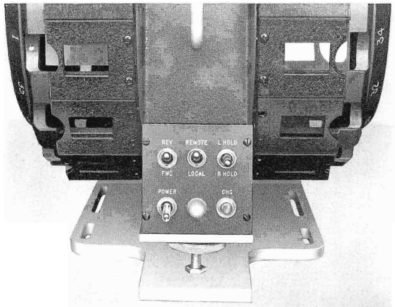
FIG. 14. All electrical controls are located at the rear of the projector. Panel includes Forward, Reverse, Hold, Power, and Change controls for completely versatile operation.
