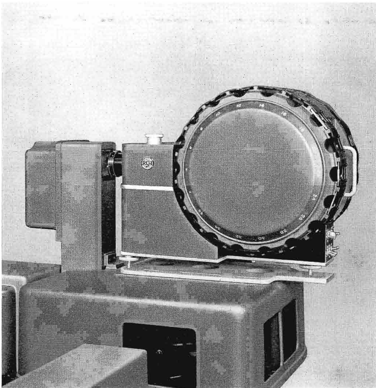
FIG. 3. Another example of versatile systems applications of the TP-7 Slide Projector. Here it is used with the periscope attachment of the TP-15 Multiplexer.
