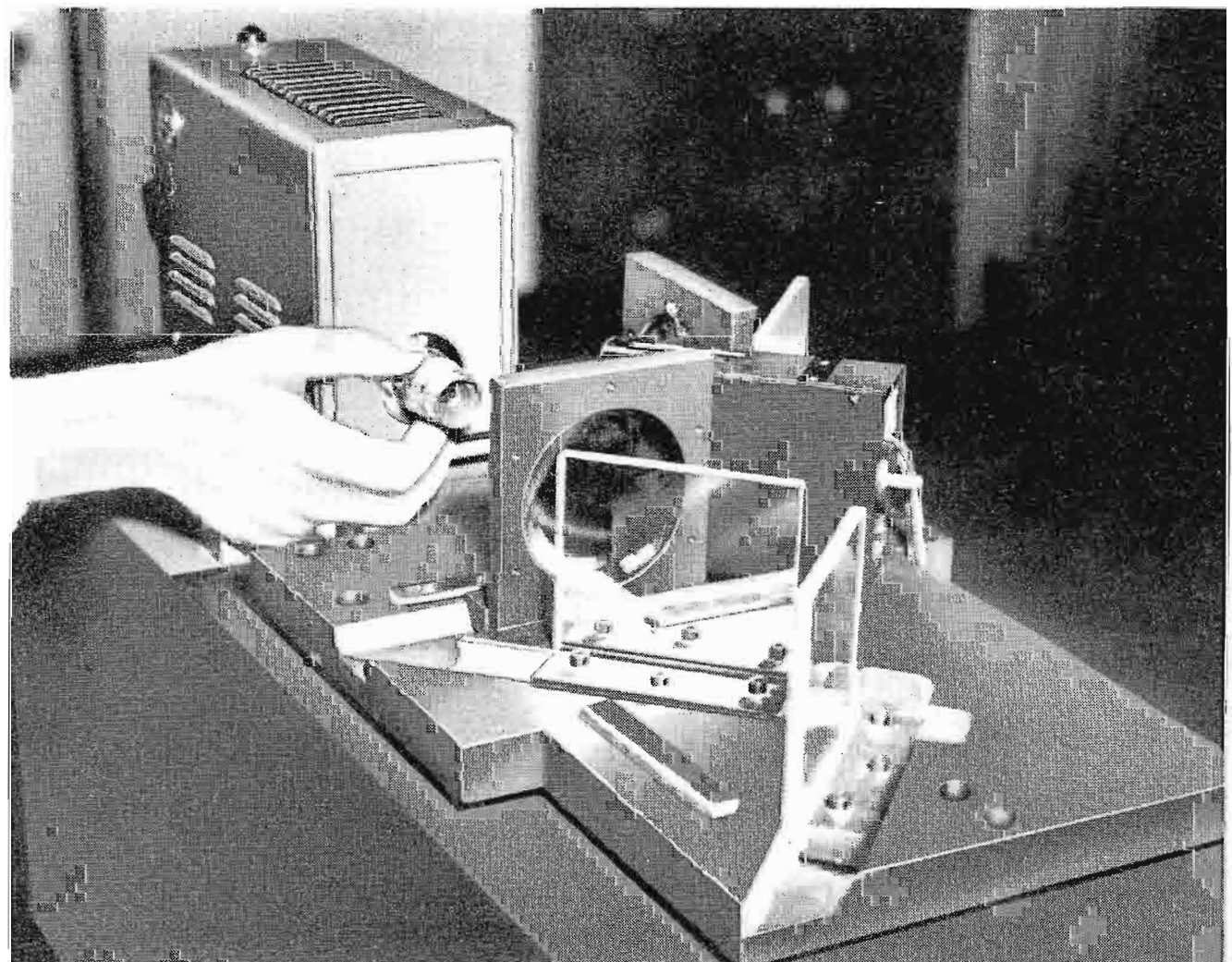
FIG. 3. TP-11 Multiplexer with cover removed.
