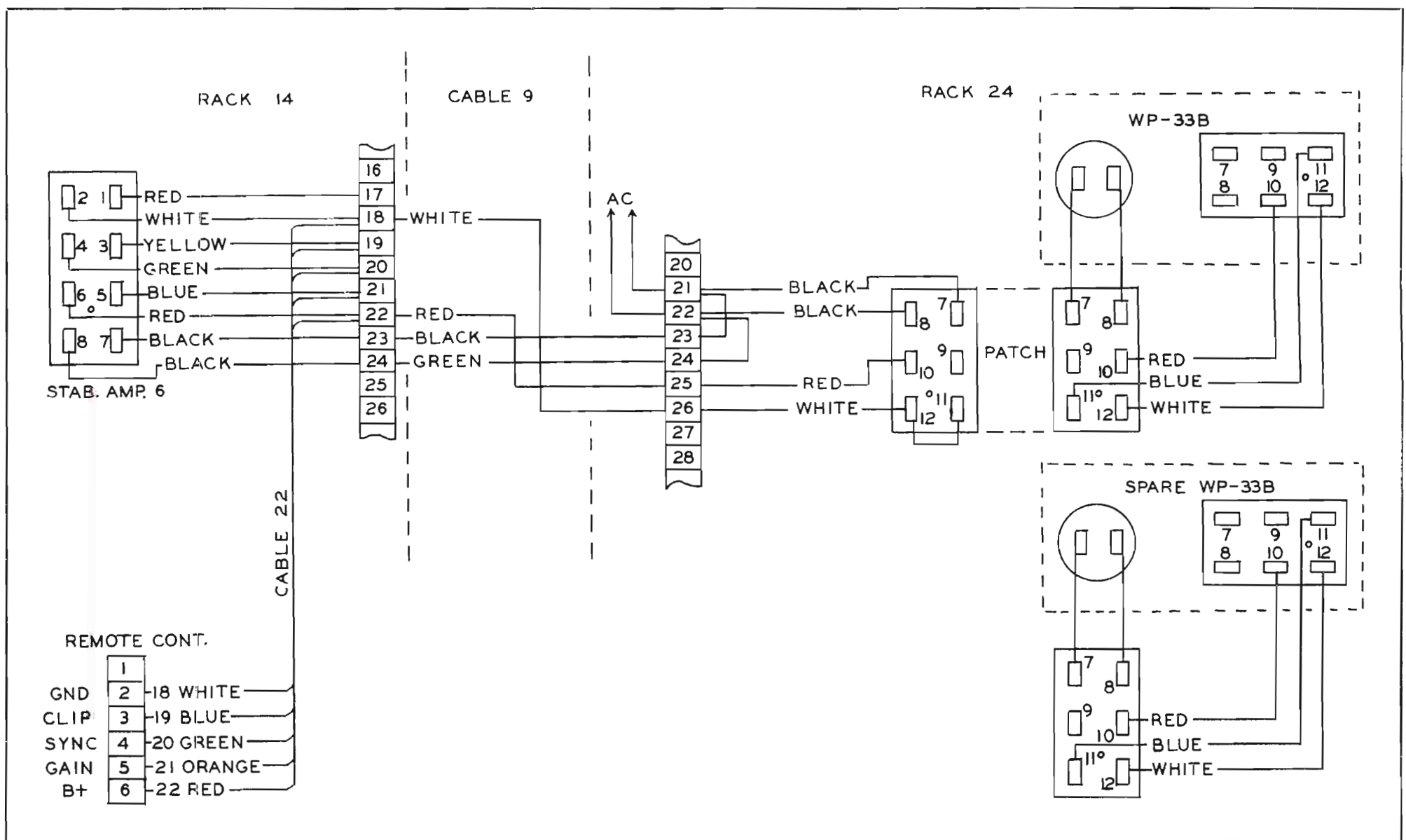
FIG. 24. Wiring diagram of power-supply patch system.
