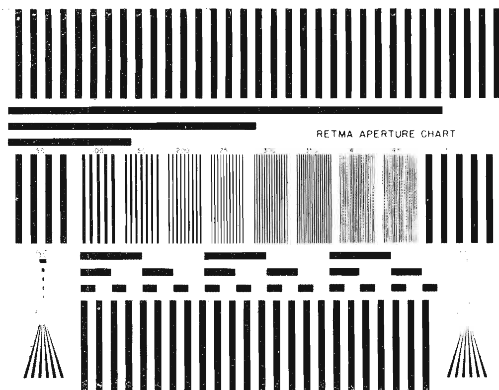
FIG. 14. RETMA Aperture Test Chart.
