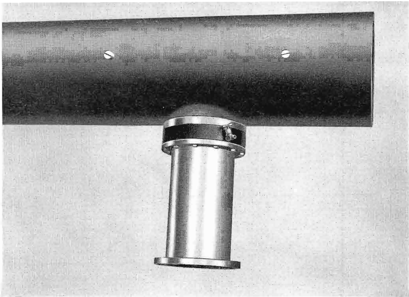
FIG. 11. Input tee of a Traveling Wave Antenna showing the location of gas stop right next to the pole. The antenna is not pressurized, but drainage holes are provided to take care of any condensation within the pole.
