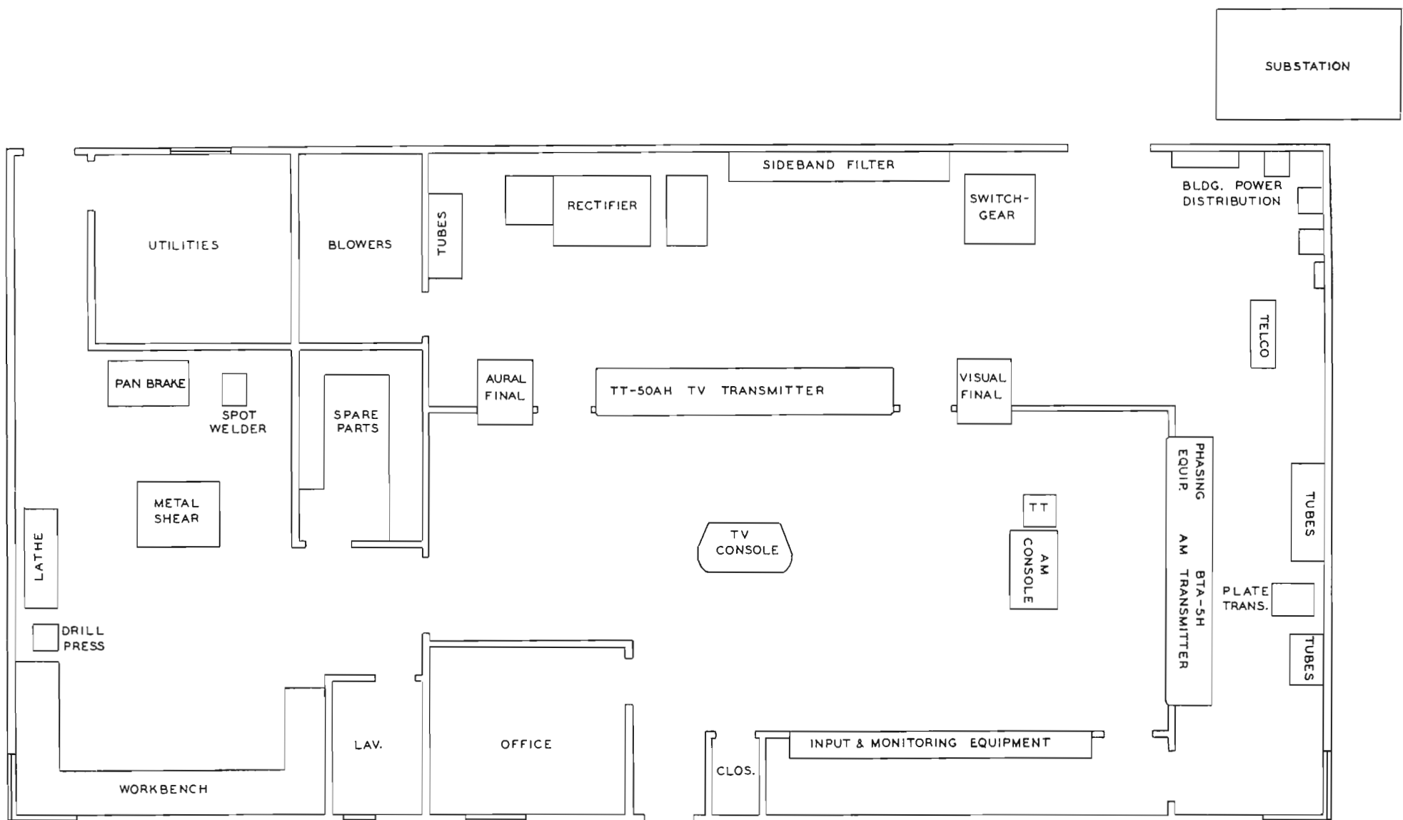
FIG. 1. Transmitter building floor plan.
