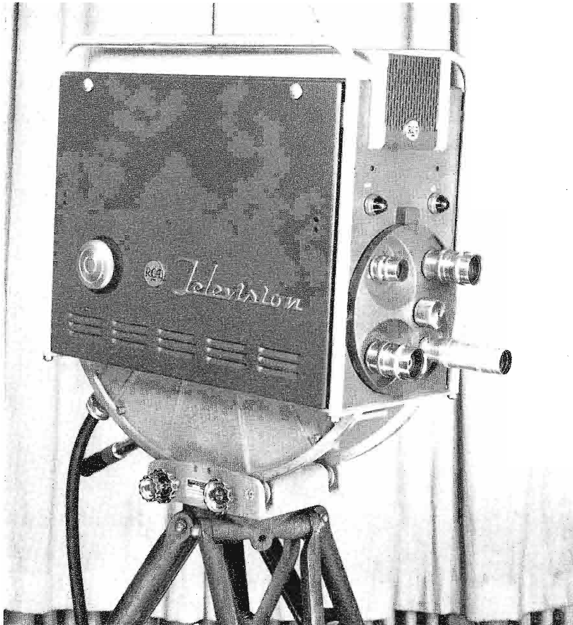
FIG. 1. Vidicon Studio Camera, Type TK-15, offers operating economy of the vidicon tube in a camera designed to broadcast standards. This new camera features a built-in 7 inch viewfinder and 4-lens turret for broadcast operations.
