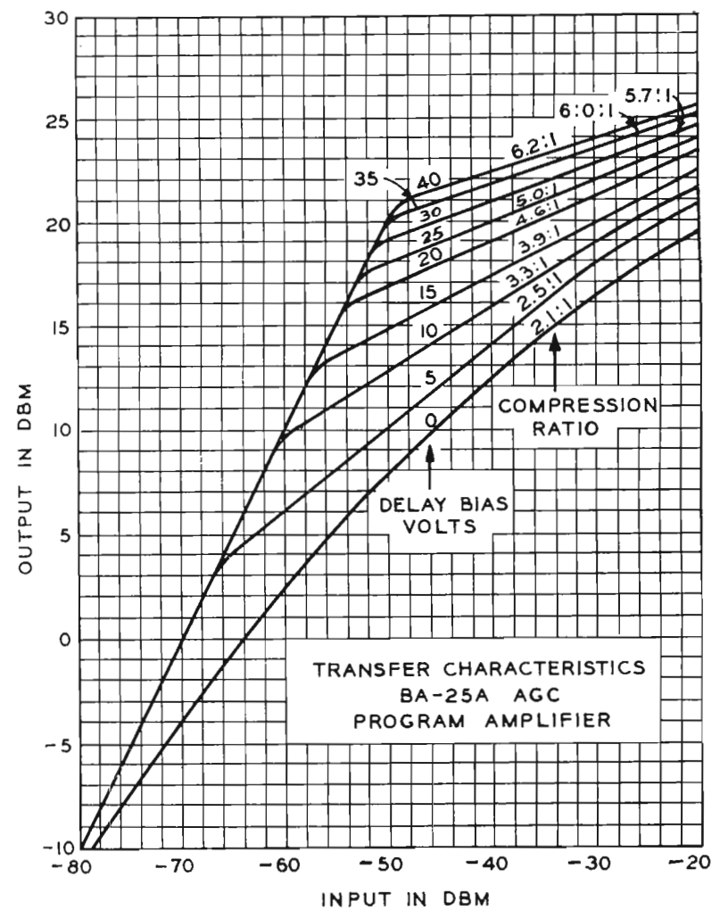
FIG. 3. Output versus input curves for the BA-25A amplifier for various values of positive delay bias.
