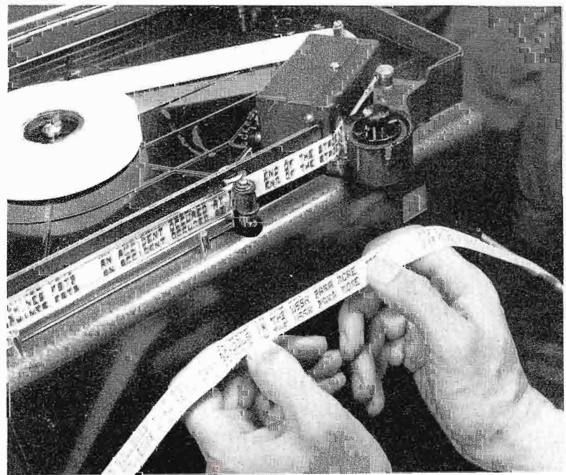
FIG. 21. Typical output of a Hellschreiber recorder. This is being fed from an RCA Communications receiver. The monitoring output at Schleissheim is fed to Munich via telephone lines.
