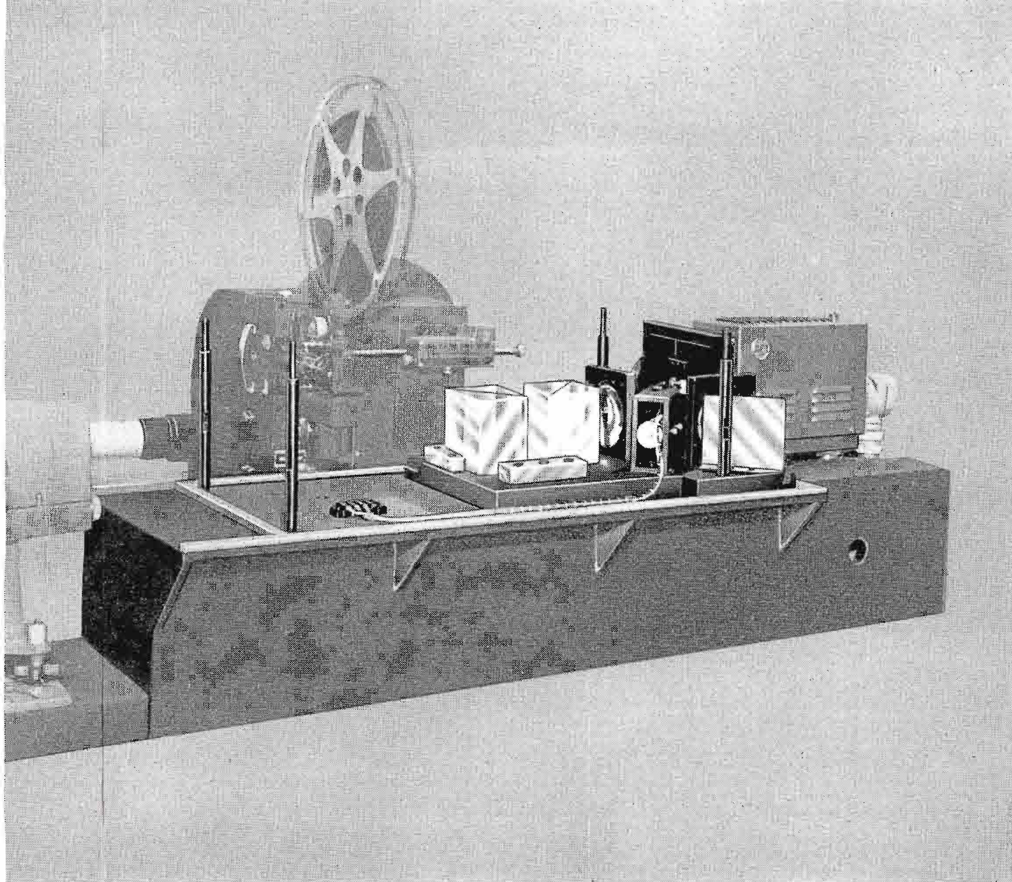
FIG. 4. TP-11B Multiplexer with cover removed.
