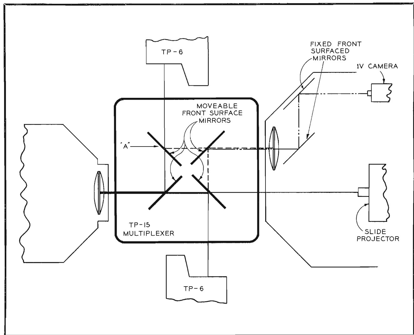
FIG. 6. Optical schematic of TP-15 Multiplexer.
