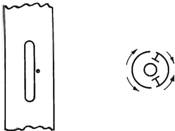
FIG. 6. Slots being used in pairs and fed in opposite phases to provide radiation similar to that of a dipole. The use of slots simplifies coupling network by allowing utilization of capacitive coupling, also eliminates protruding radiators and makes possible lesser wind load.
