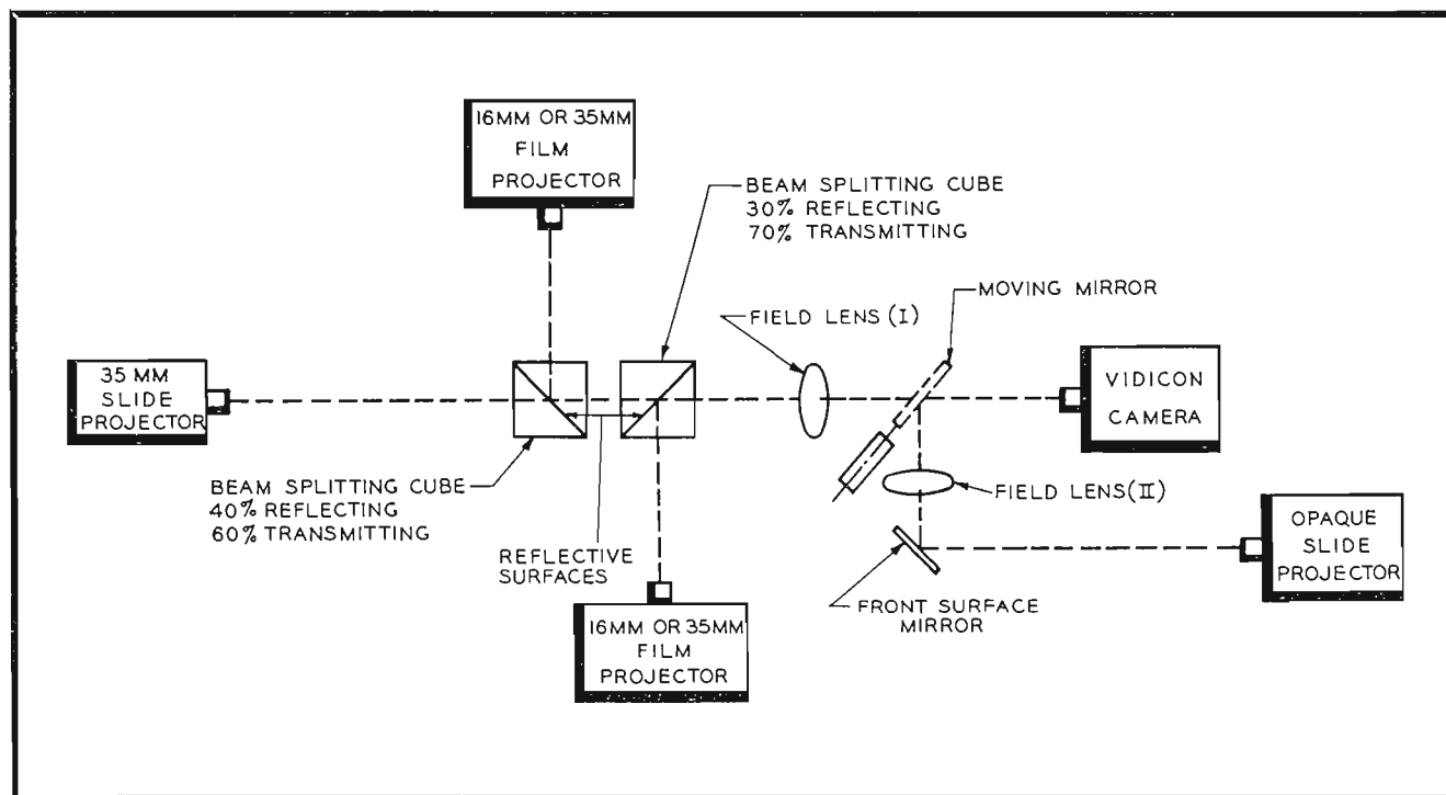
FIG. 5. Optical schematic of TP-11B Multiplexer.
